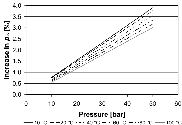
Figure 2. Deviations between water partial pressures in saturated humid air calculated with the common idealised model and partial pressures calculated considering a first order correction.
